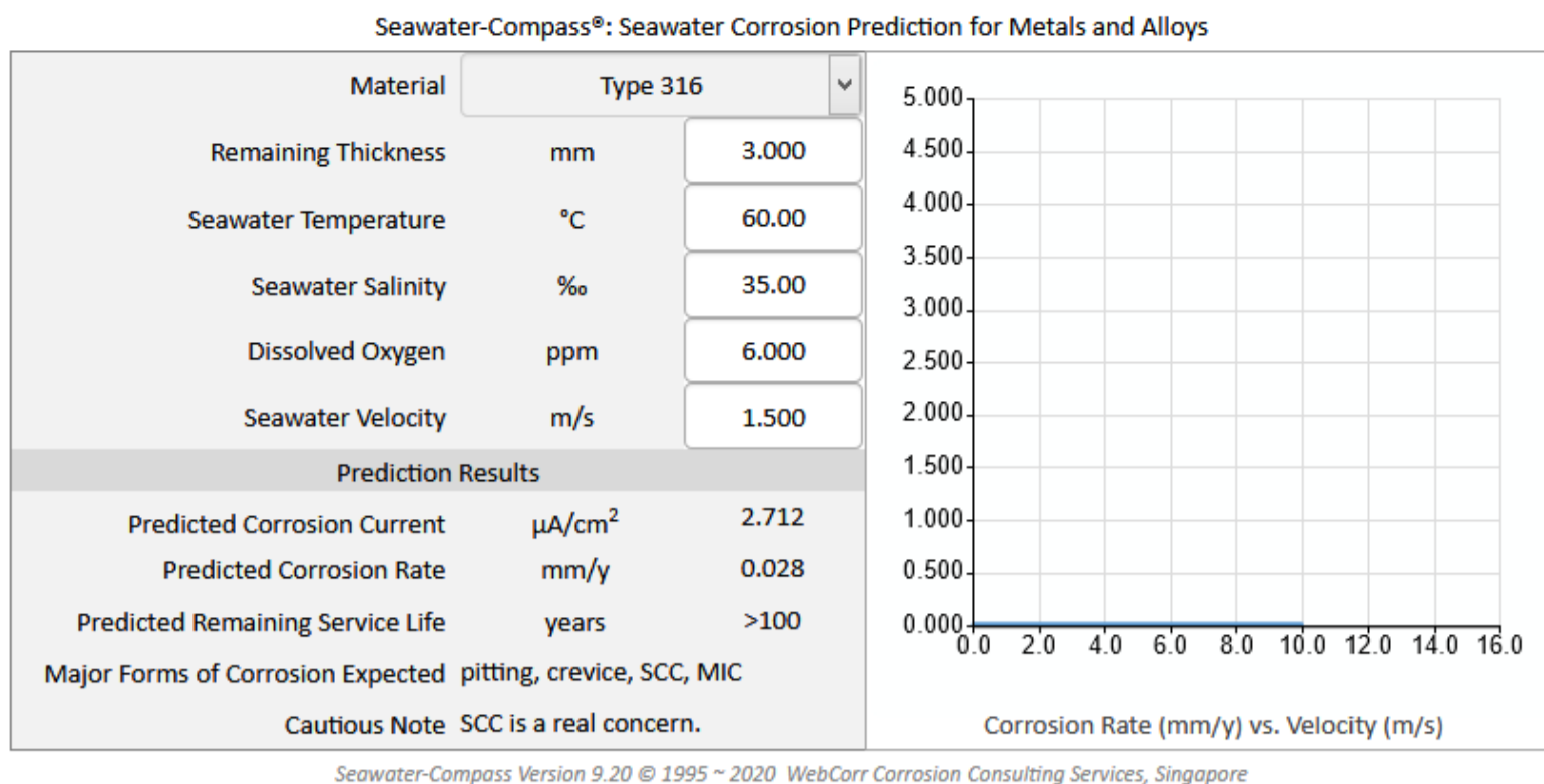
Figure 4 Seawater-Compass predicts the risk of stress corrosion cracking (SCC) of austenitic stainless steels in seawater services.
